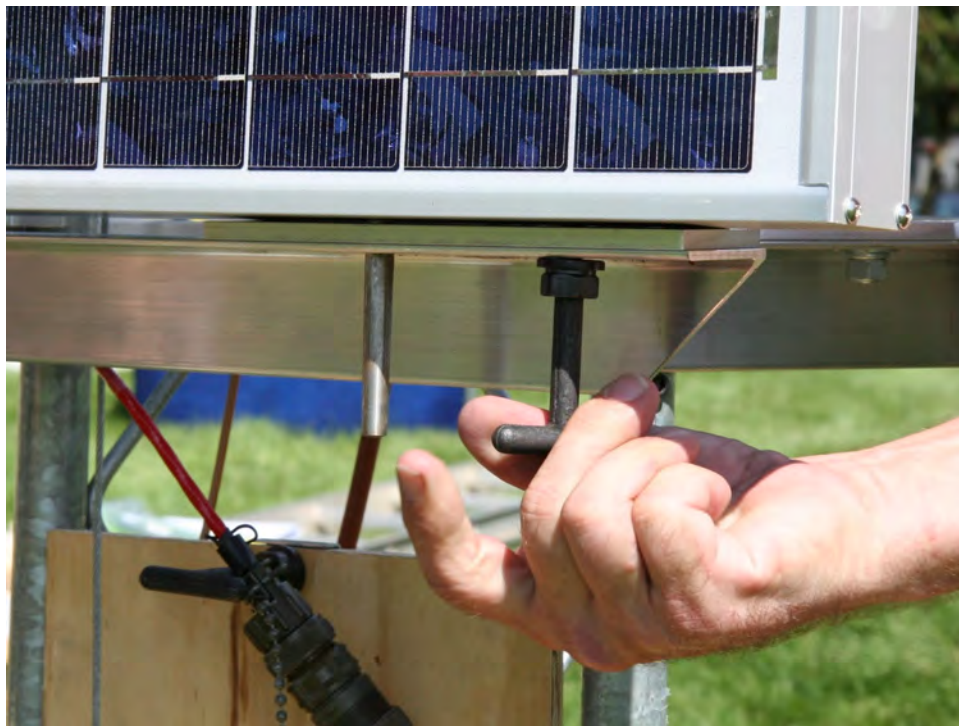
Figure 14. T-bolts used for solar panel assembly.
