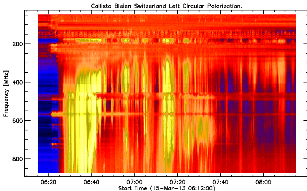
Fig. 6: Two hours of observation at Bleien observatory. Strong activity mainly in LHCP. RHCP burst activity is relatively low. Blue color means no burst, only background noise. Red means hot and yellow denotes to very hot radiation. Horizontal structures denote to strong local radio interference from DVB-T.
