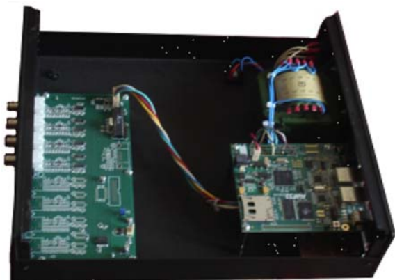
Figure 3. SEVAN DAQ module.
