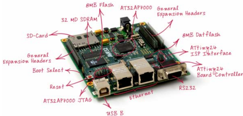
Figure 4. ATNGW100 Network Gateway Kit.
