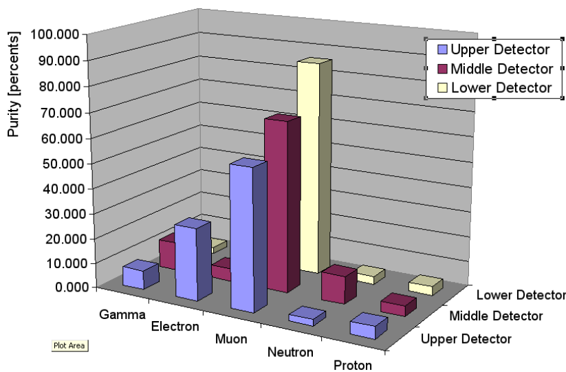
Figure 6. The purity of 3 SEVAN layers.
