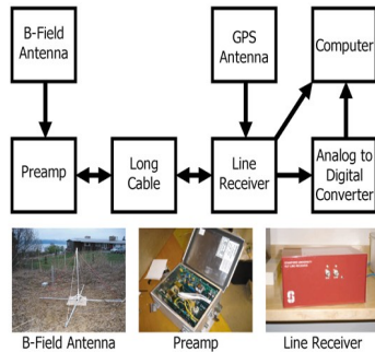
Figure I Very low frequency data acquisition system
