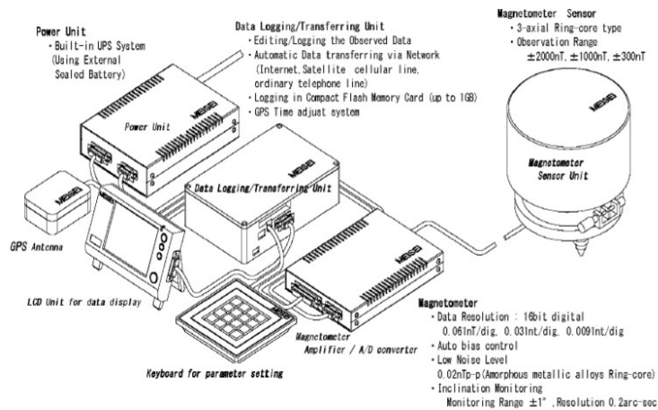
Figure II MAGDAS/CPM magnetometer system for real-time data acquisition
